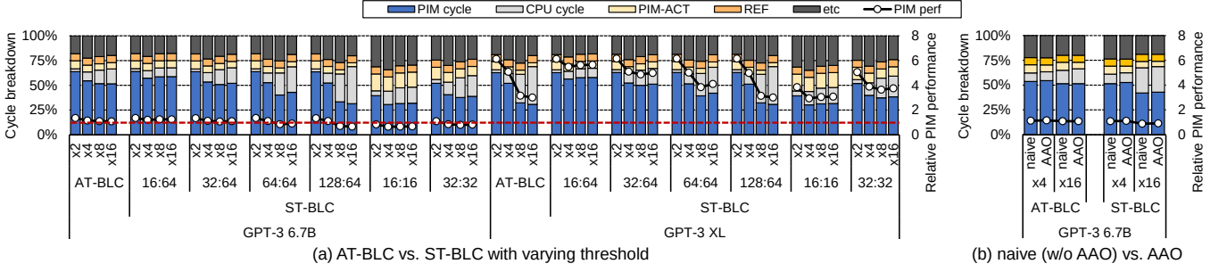
Figure 10: Memory cycle breakdown and PIM performance on LPDDR-PIM with (a) AT-BLC and ST-BLCs with varying threshold values; the threshold values for N and P of ST-BLC are indicated on the x-axis as N:P , and (b) without AAO (naive), under different CPU program counts ( \times N ). PIM performance is normalized to the target QoS (the red dotted line).
