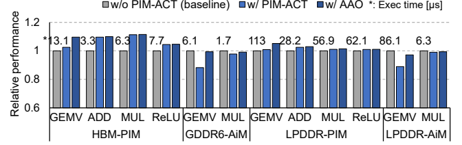
Figure 7: PIM microbenchmarks performance in HBM-PIM, GDDR6-AiM, LPDDR-PIM and LPDDR-AiM with PIM-ACT.
