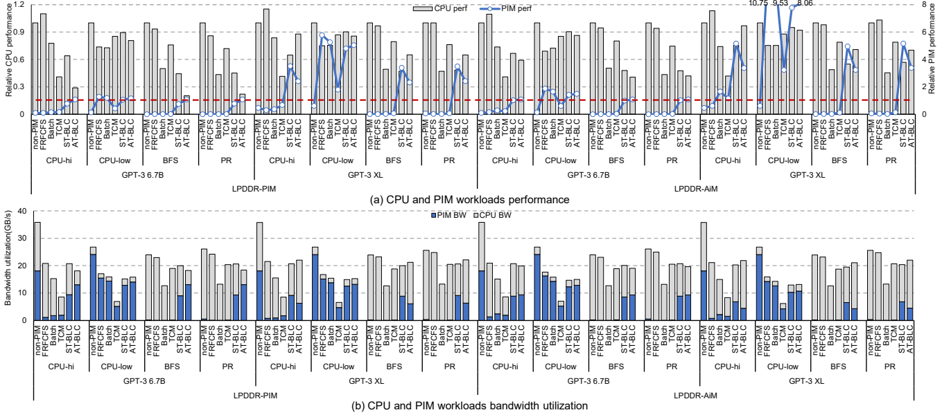
Figure 8: (a) Performance and (b) bandwidth utilization of PIM and CPU workloads in LPDDR-PIM and LPDDR-AiM systems with ComPASS under different scheduling policies. FR-FCFS, Batch, TCM, ST-BLC, and AT-BLC execute GPT-3 GEMV on PIM, while non-PIM runs them on the host processor. PIM performance is the inverse of execution time, normalized against the target execution time required to meet the QoS (the red dotted line).
