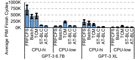
Figure 9: Mean and standard deviation of PIM operation (GEMV) execution times across MCs under different schedulers on LPDDR-PIM.
