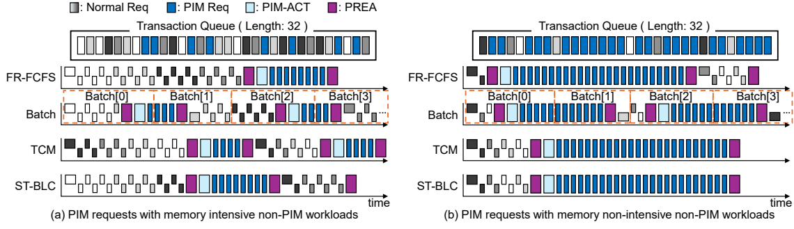
Figure 6: Scheduling policy comparison under PIM/non-PIM co-execution. Normal requests from different threads are shown in different shades of gray. PIM requests, PIM-ACT, and PREA commands are shown in blue, light blue, and purple, respectively.
