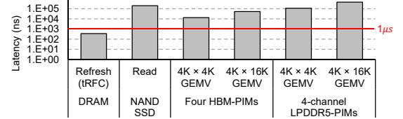
Figure 2: Comparison of PIM-based GEMV execution time, DRAM refresh, and NAND-based SSD read latency.
