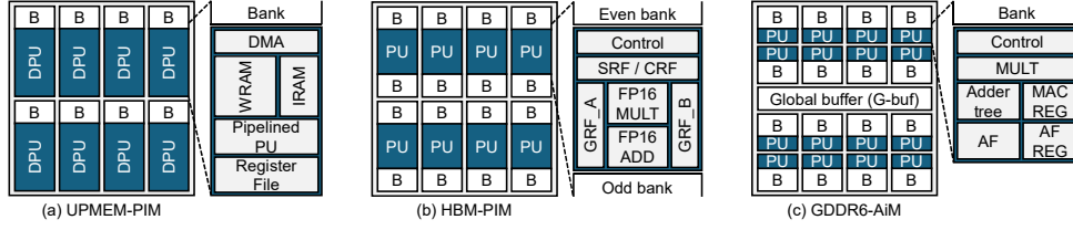
Figure 1: Existing real-world PIM architectures.
