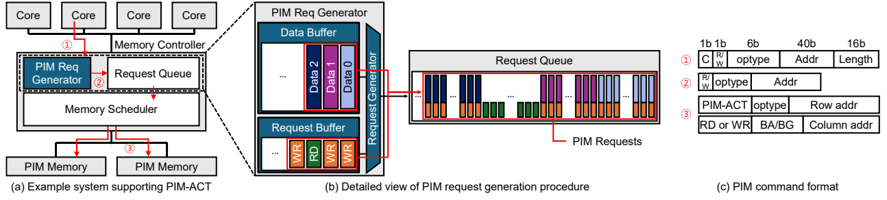
Figure 4: Memory system with PIM request generator, which contains request buffer and data buffer to store PIM macro requests and data for PIM operations, respectively. Request generator decodes PIM macro requests and generates PIM micro requests.
